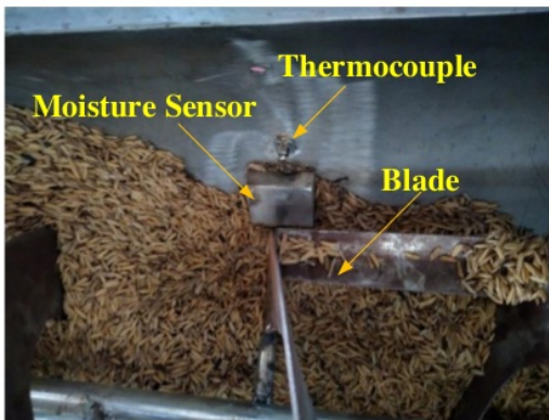
Figure 9. Installation of the thermocouple sensor and moisture sensor
