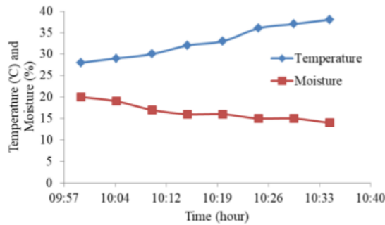
Figure 17. Graph of Temperature rate and grain moisture
