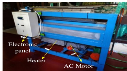
Figure 7. Mechanical of grain drying machine
