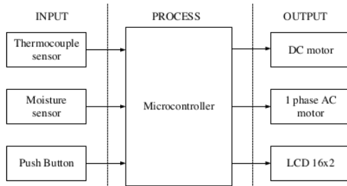
Figure 1. Blok diagram system
