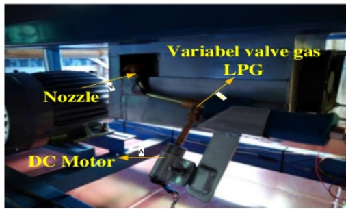
Figure 8. Heater System with LPG Gas
