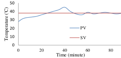
Figure 16. Third tested with K_p=2 , K_i=2 , K_d=10
