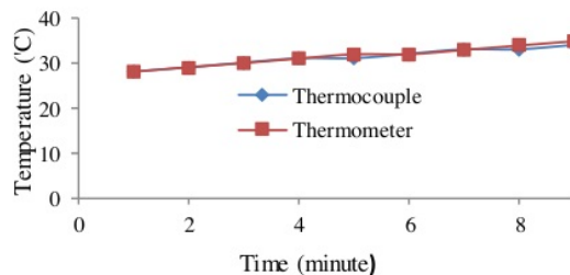
Figure 10. Graph of thermocouple sensor testing
