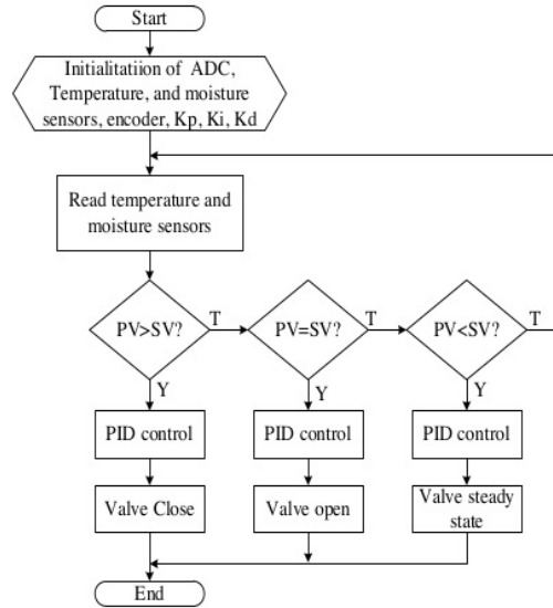
Figure 6. Drying machine flowchart
