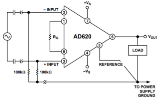
Figure 2. Thermocouple gain circuit
