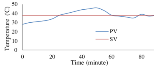
Figure 15. Second tested with K_p=3 , K_i=1 , K_d=6
