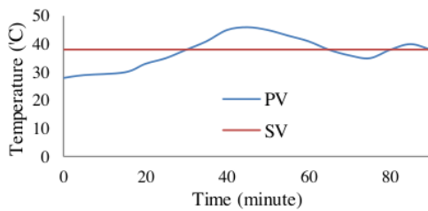
Figure 14. First tested with K_p=3 , K_i=1 , K_d=6
