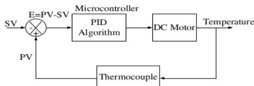
Figure 5. Controlling system block diagram
