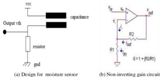
Figure 3. The Moisture Sensor
