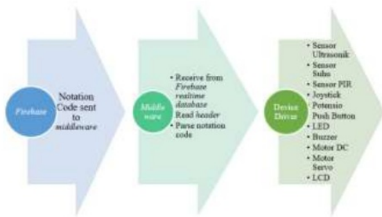
Figure 3. Workflow system
