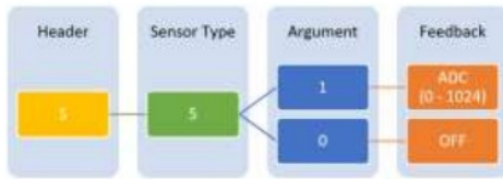
Figure 9. Potensiometer access notation
