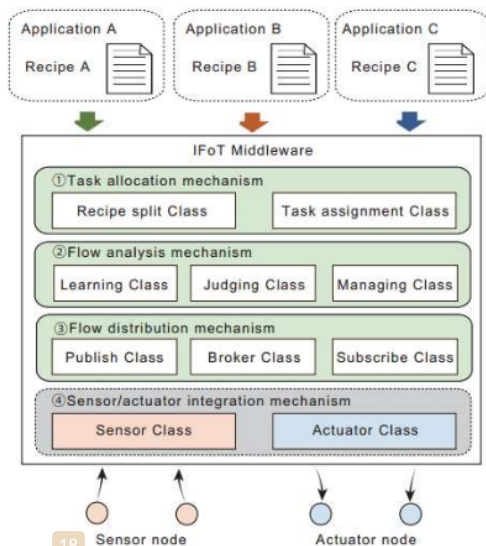
Figure 1. The logic architecture of the IFoT middleware
