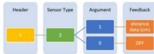
Figure 6. Distance sensor access notation
