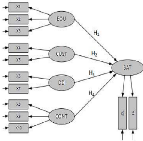
Figure 2. Path analysis
