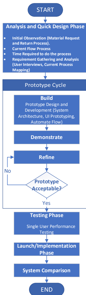
Fig.3. Research Framework
